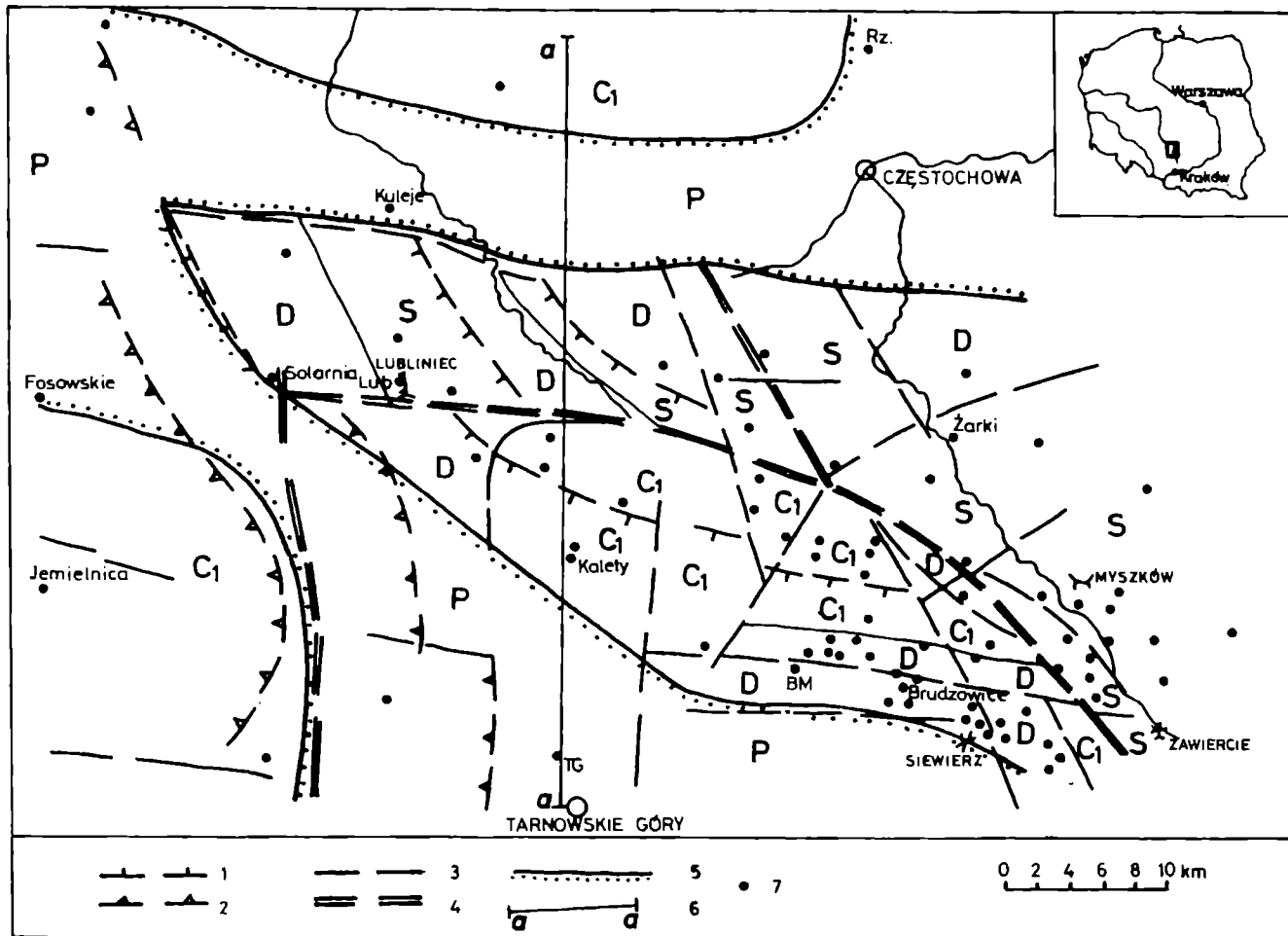
Fig. 2. Geologic sketch map of the top of the Paleozoic series based on the interpretation of gravimetric and satellite lineaments (after Fig. 4). 1 – thrusts; 2 – Culm overthrusts; 3 – faults; 4 – deep fractures; 5 – extent of Permian deposits; 6 – cross-section line (see Fig. 3); 7 – important boreholes: Rz – Rzeki IG1, Kul – Kuleje IG1, Solar – Solarnia IG1, Lub – Lubliniec IG1, Kal – Kalety IG1, BM – BM 152; S – Silurian; D – Devonian; C 1 – lower Carboniferous; P – Permian
